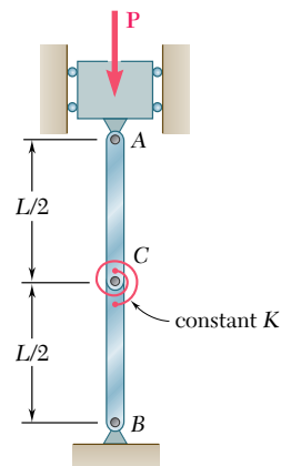
Fig. 10.3 Column model.
