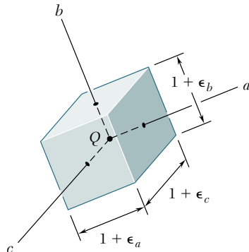
Fig. 7.67 Principal strains.
