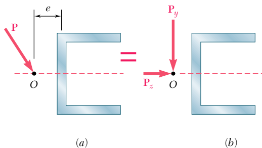
Fig. 6.47 Beam with oblique load.
