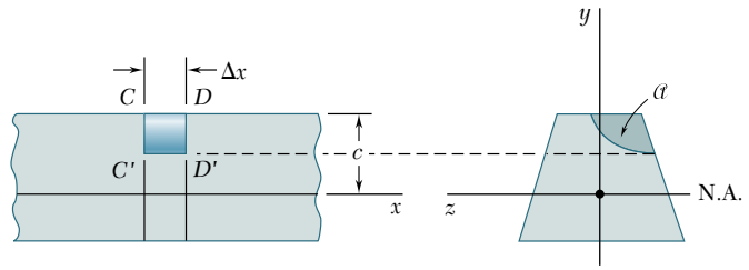
Fig. 6.23 Short segment of beam example.
