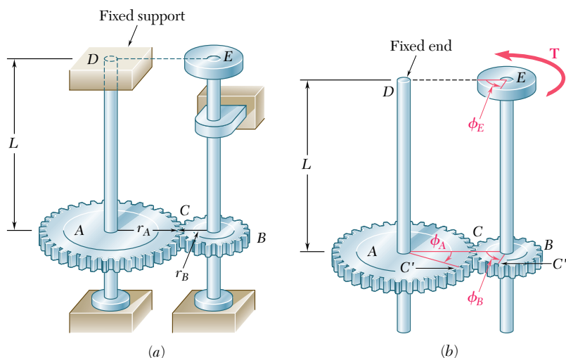
Fig. 3.23 Gear assembly.
