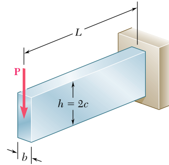
Fig. 6.17 Cantilever beam.
