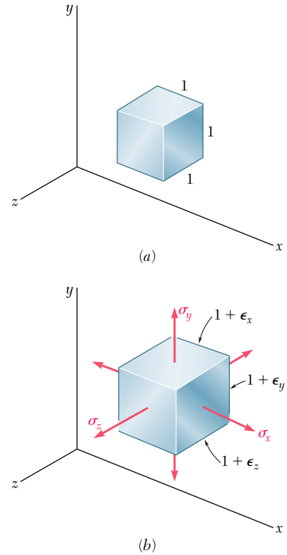
Fig. 2.39 Deformation of cube under multiaxial loading.
