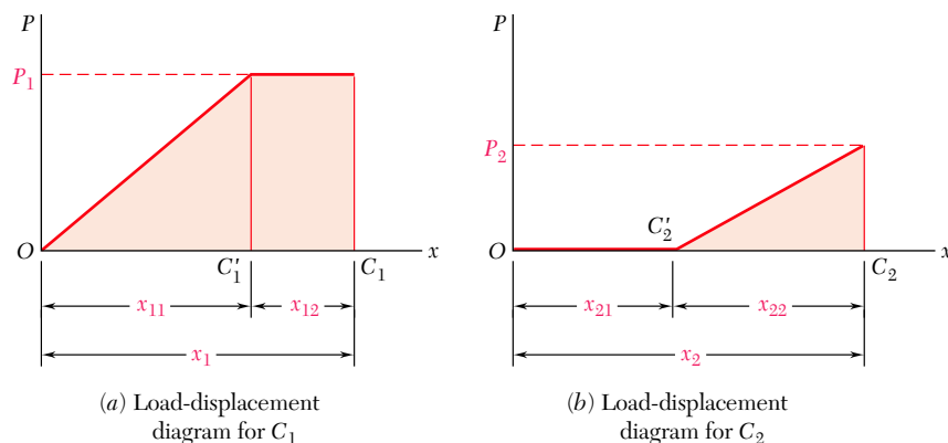
Fig. 11.37 Load-displacement diagrams.
