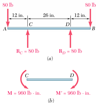
Fig. 4.2 Beam in which portion CD is in pure bending.
