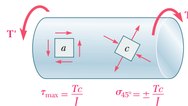
Fig. 3.58 Angle of twist
