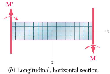
Fig. 4.9 Member subject to pure bending.
