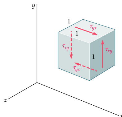
Fig. 2.42 Cubic element subjected to shearing stresses.
