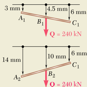
(a) Deflections for \delta_B = 10 \text{ mm} ◀
