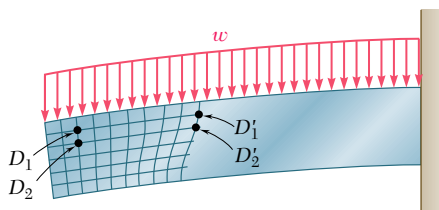
Fig. 6.21 Deformation of cantilever beam with distributed load.
