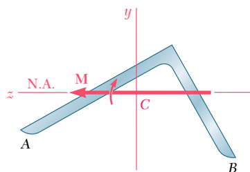
Fig. 6.55 Beam without plane of symmetry.
