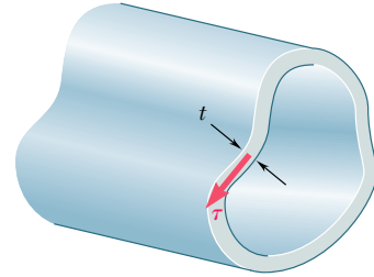
Fig. 3.51 Direction of shearing stress on cross section.
