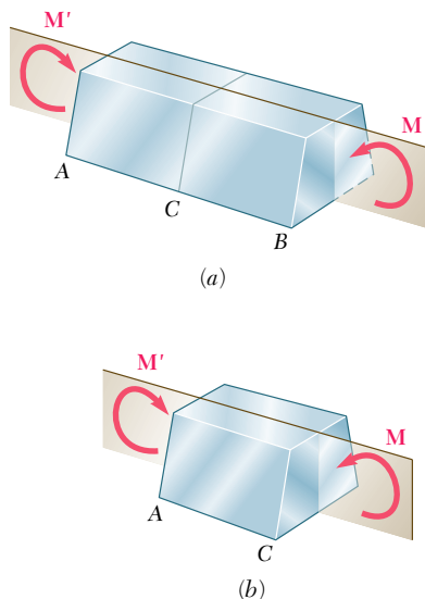
Fig. 4.5 Member in pure bending.
