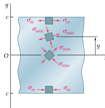
Fig. 8.6 Principal stresses at selected points of a beam.
