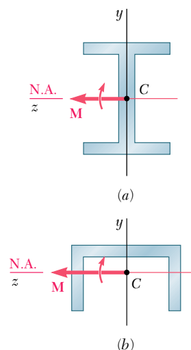
Fig. 4.49 Moment in plane of symmetry.
