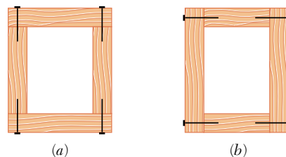
Fig. 6.22 Box beam cross sections.
