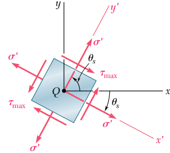
Fig. 7.10 Maximum shearing stress.
