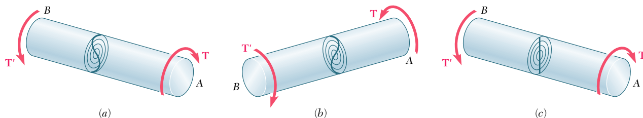
Fig. 3.11 Potential deformations of cross section.
