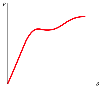
Fig. 2.2 Load-deformation diagram.
