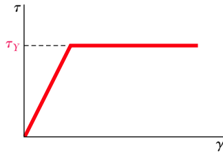
Fig. 3.34 Elastoplastic stress-strain diagram.
