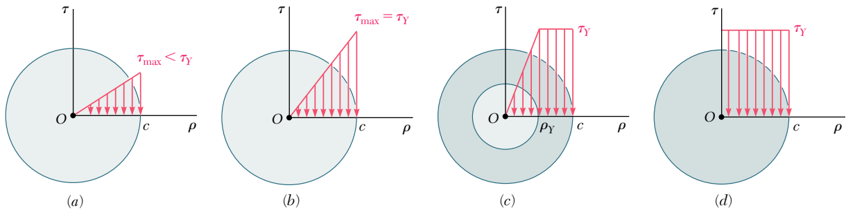
Fig. 3.35 Stress distributions for shaft made of elastoplastic material.
