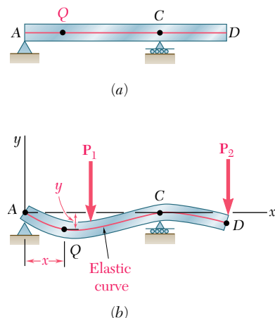
Fig. 9.6 Elastic curve for beam of Fig. 9.4.
