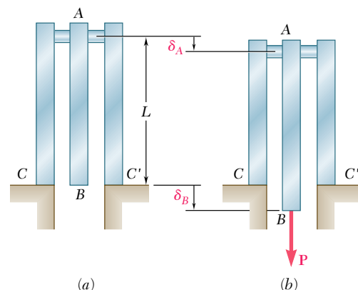
Fig. 2.20 Example of relative end displacement, as exhibited by the middle bar.
