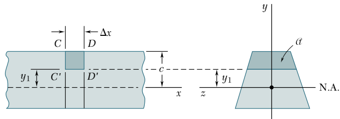
Fig. 6.5 Short segment of beam example.
