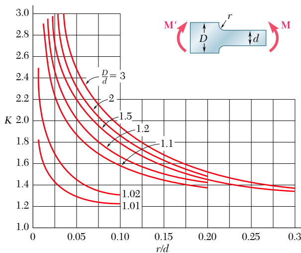
Fig. 4.27 Stress-concentration factors for flat bars with fillets under pure bending. †
