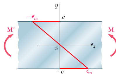
Fig. 4.30 Linear strain distribution in beam.
