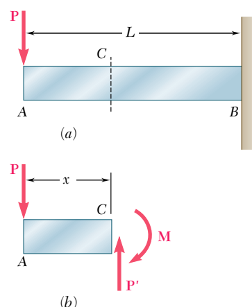
Fig. 4.4 Cantilever beam, not in pure bending.
