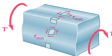
Fig. 3.44 Deformation of square bar.
