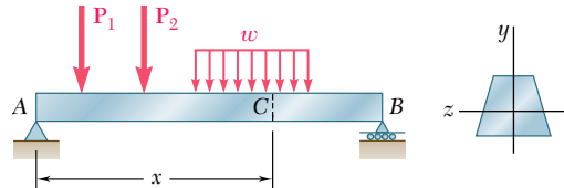
Fig. 6.4 Beam example.
