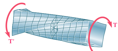
Fig. 3.42 Twisting of shaft with square cross section.
