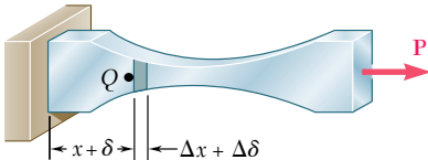
Fig. 2.5 Deformation of axially-loaded member of variable cross-sectional area.
