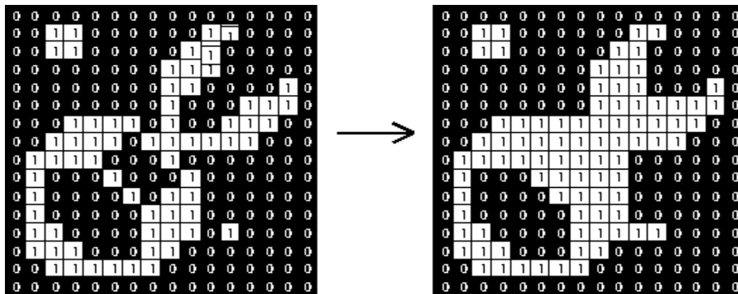
Fig: Effect of closing using a 3×3 square structuring element
