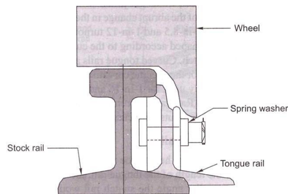
Fig. Overriding switch
