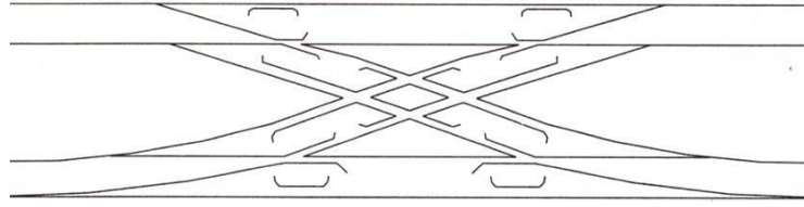
Fig. Scissors crossover
