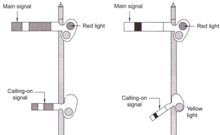
Fig. Calling-on signal
