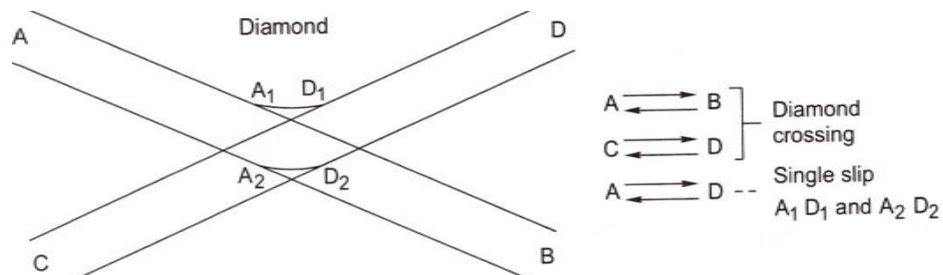
Fig. Single slip
