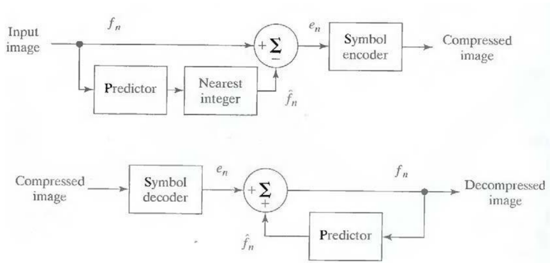
Fig.8.1 A lossless predictive coding model: (a) encoder; (b) decoder
