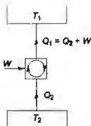
Fig. 14.2 Reversed heat engine cycle
