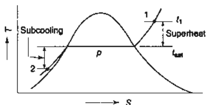
Fig. 9.19 Superheat and subcooling
