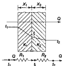
Fig. 18.4 Heat conduction through resistance in series
