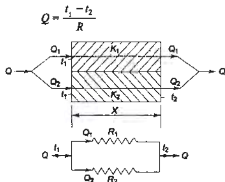
Fig. 18.5 Heat conduction through resistance in parallel
