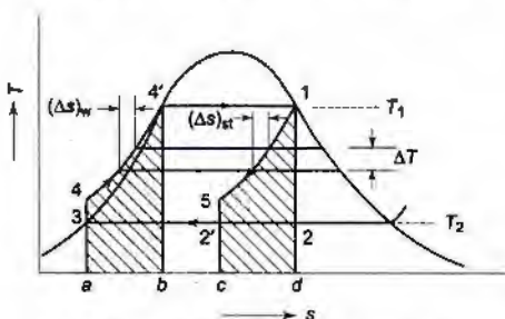
Fig. 12.17 Ideal regenerative cycle on T-s plot
