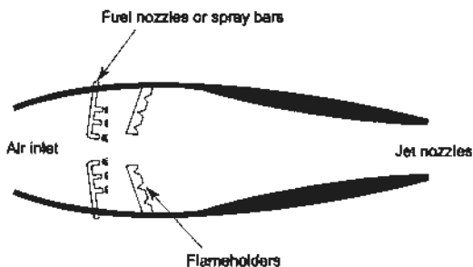
Fig. 13.30 Ramjet engine
