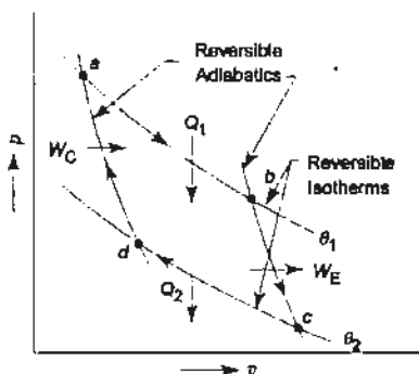
Fig. 6.31 Carnot cycle of an ideal gas
