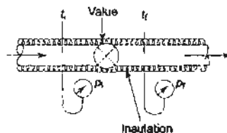
Fig. 11.2 Joule-Thomson expansion
