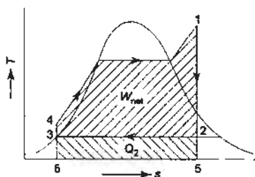
Fig. 12.6 Q_1 , W_{\text{net}} and Q_2 are proportional to areas
