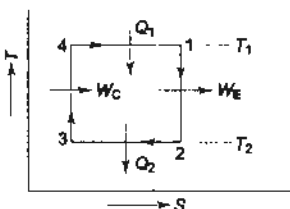
Fig. 7.9 Carnot cycle
