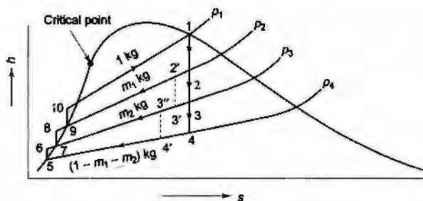
Fig. 12.21 Regenerative cycle on h - s diagram
