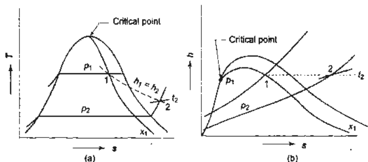
Fig. 9.24 Throttling process on T - s and h - s plots
