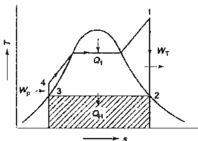
Fig. 12.33 By-product power cycle
