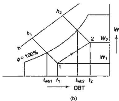
Fig. 15.9 Heating and humidification
