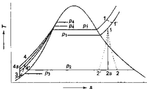
Fig. 12.8 Various losses on T-s plot
