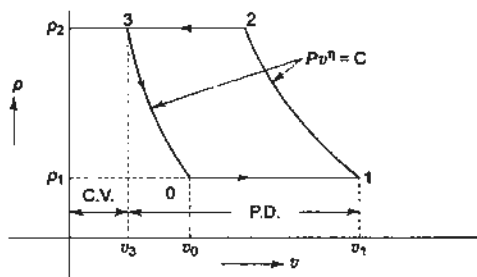
Fig. 10.5 Processes in an idealized reciprocating compressor
