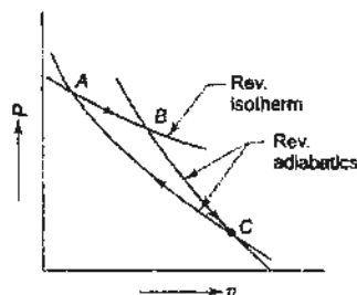
Fig. 7.1 Assumption of two reversible adiabatics intersecting each other
