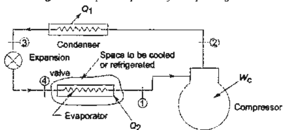
Fig. 14.8 Vapour compression plant
