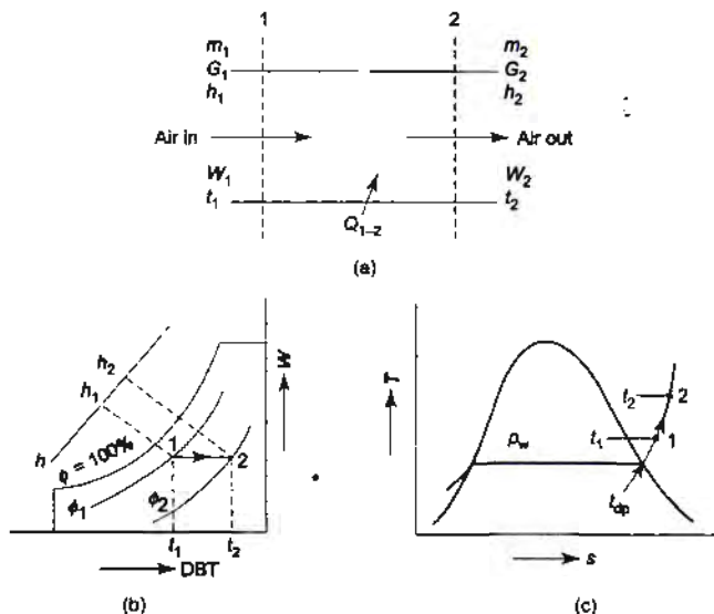
Fig. 15.6 Sensible heating
