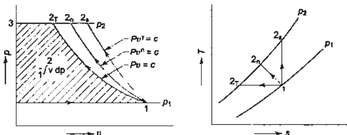
Fig. 10.3 Reversible compression processes
