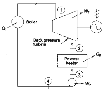
Fig. 12.32 Back pressure turbine
