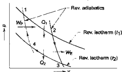
Fig. 6.21 Carnot cycle
