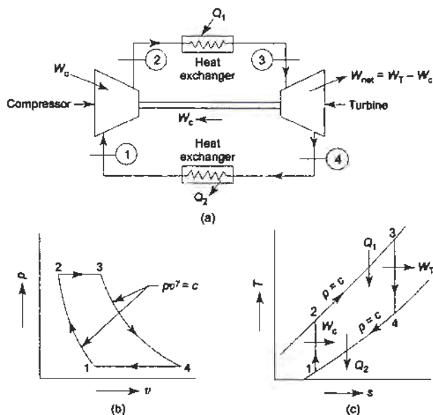
Fig. 13.13 (a-c) Brayton cycle
