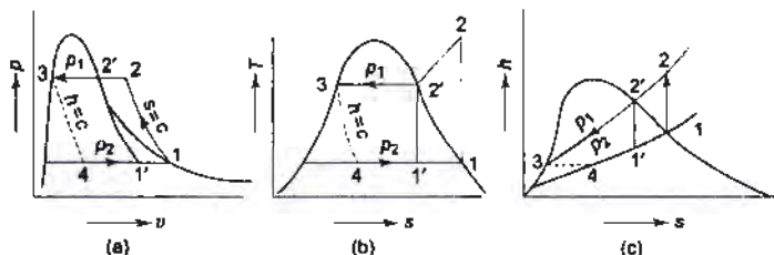
Fig. 14.5 Vapour compression refrigeration cycle-property diagrams
