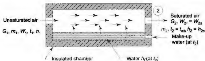
Fig. 15.3 Adiabatic saturation process
