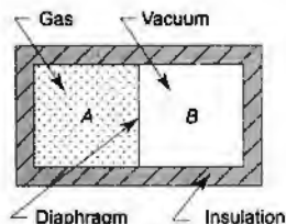
Fig. 6.14 Free expansion
