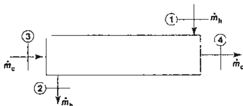
Fig. 8.22 Exergy balance of a heat exchanger
