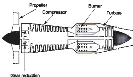
Fig. 13.29 Turboprop engine
