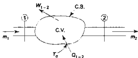
Fig. 8.16 Exergy balance for a steady flow system
