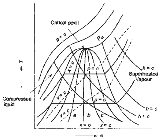
(a) Constant property lines on T - s plot
