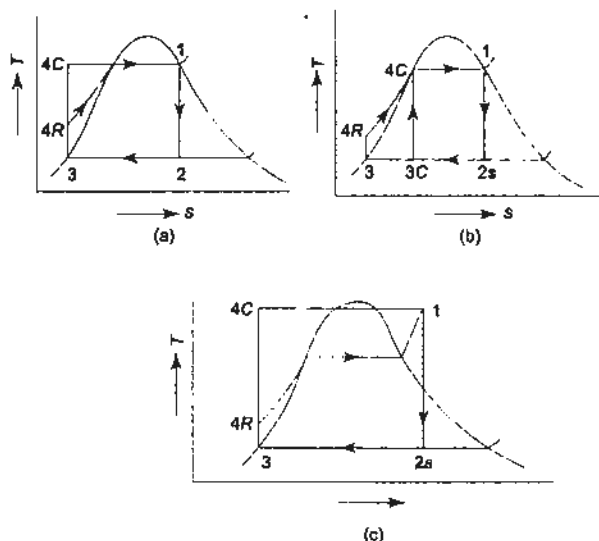
Fig. 12.9 Comparison of Carnot and Rankine cycles
