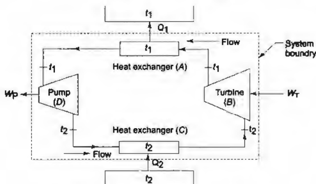
Fig. 6.23 Reversed Carnot heat engine-steady flow process
