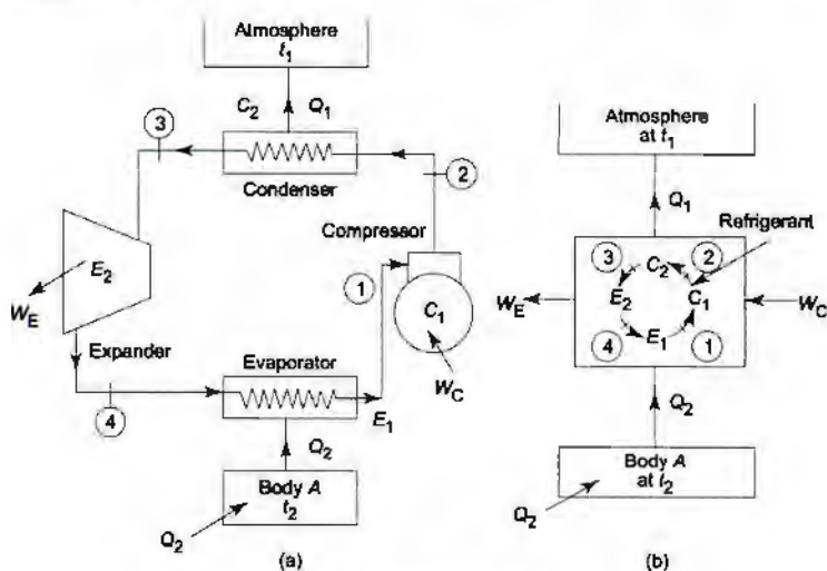
Fig. 6.7 A cyclic refrigeration plant
