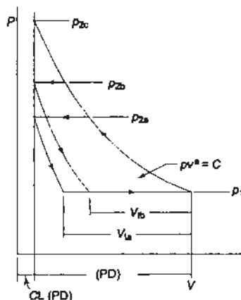
Fig. 10.7 Effect of pressure ratio on capacity
