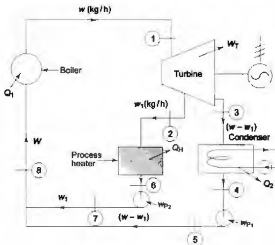
Fig. 12.34 Pass-out turbine
