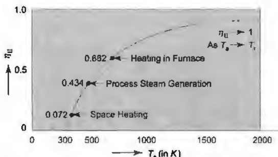
Fig. 8.20 Effect of use temperature T_s on the second law efficiency ( T_r = 2200\text{K} , T_0 = 300\text{K} , \eta_r = 100\% )
