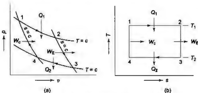
Fig. 13.1 Carnot cycle
