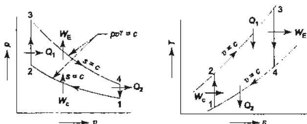
Fig. 13.5 (c) Otto cycle
