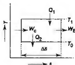
Fig. 8.4 Carnot cycle
