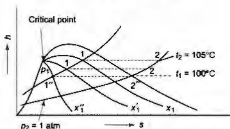
Fig. 9.25 Minimum quality that can be measured only by throttling
