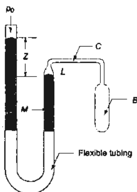
Fig. 2.1 Constant volume gas thermometer
