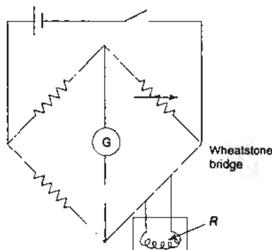
Fig. 2.3 Resistance thermometer
