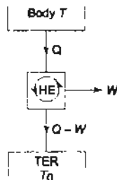
Fig. 7.18 Maximum work obtainable when one of the bodies is a TER
