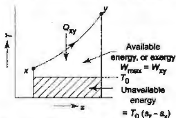
Fig. 8.3 Unavailable energy by the second law
