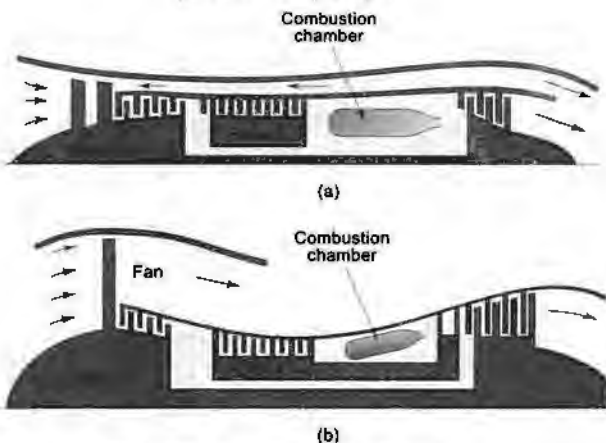
Fig. 13.28 Turbofan or bypass jet engines
