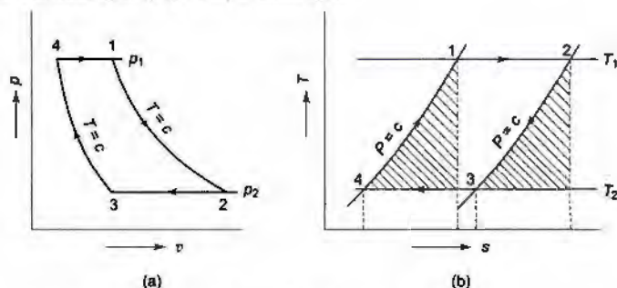
Fig. 13.3 Ericsson cycle
