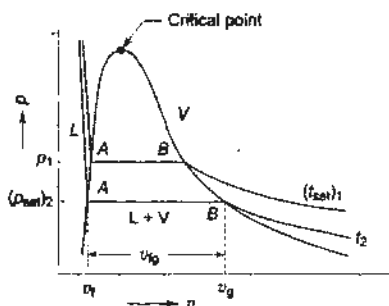
Fig. 9.7 Saturation pressure and temperature
