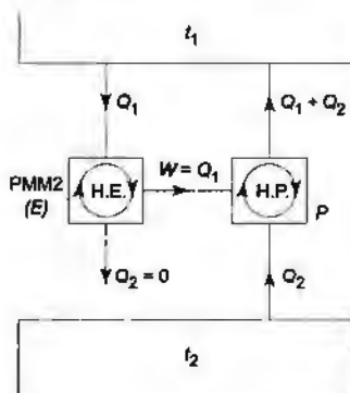
Fig. 6.10 Violation of the Kelvin-Planck statement
