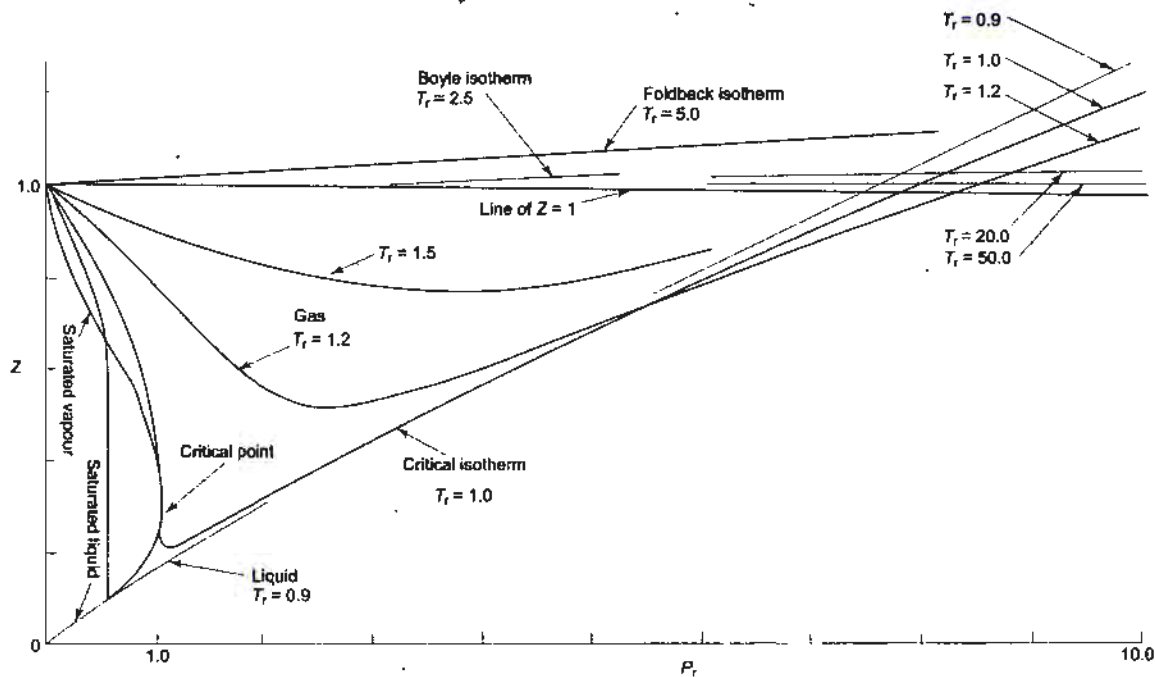
Fig. 10.10 (a) Generalized compressibility chart
