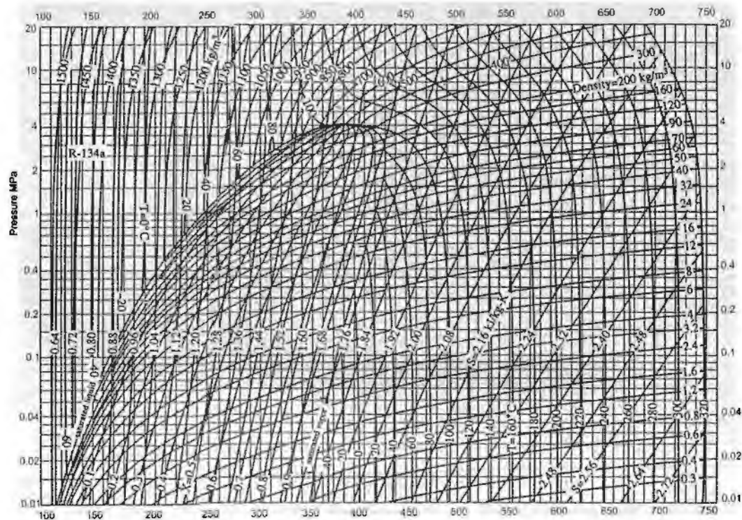
Fig. B.3 p - h diagram for refrigerant R-134a
