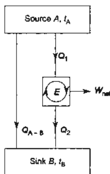
Fig. 6.12 Heat transfer through a finite temperature difference
