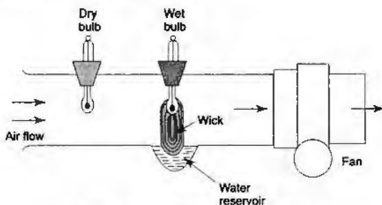
Fig. 15.2 Dry and wet bulb temperatures
