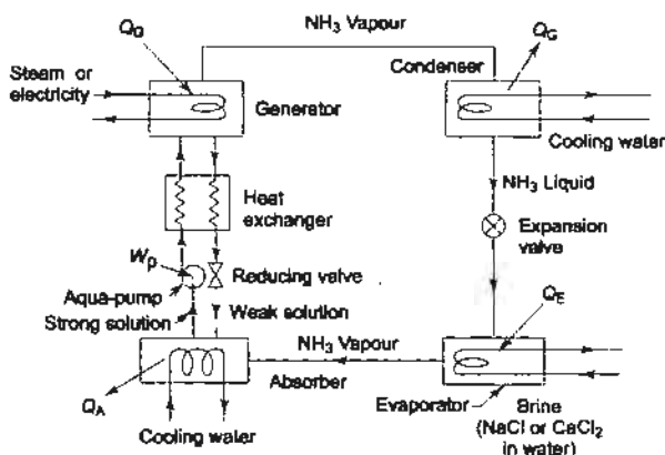
Fig. 14.15 Vapour absorption refrigeration plant-flow diagram
