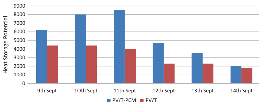
Fig. 7.7 Daily heat storage potential of PVT-PCM and PVT-water systems (Browne et al. 2015)
