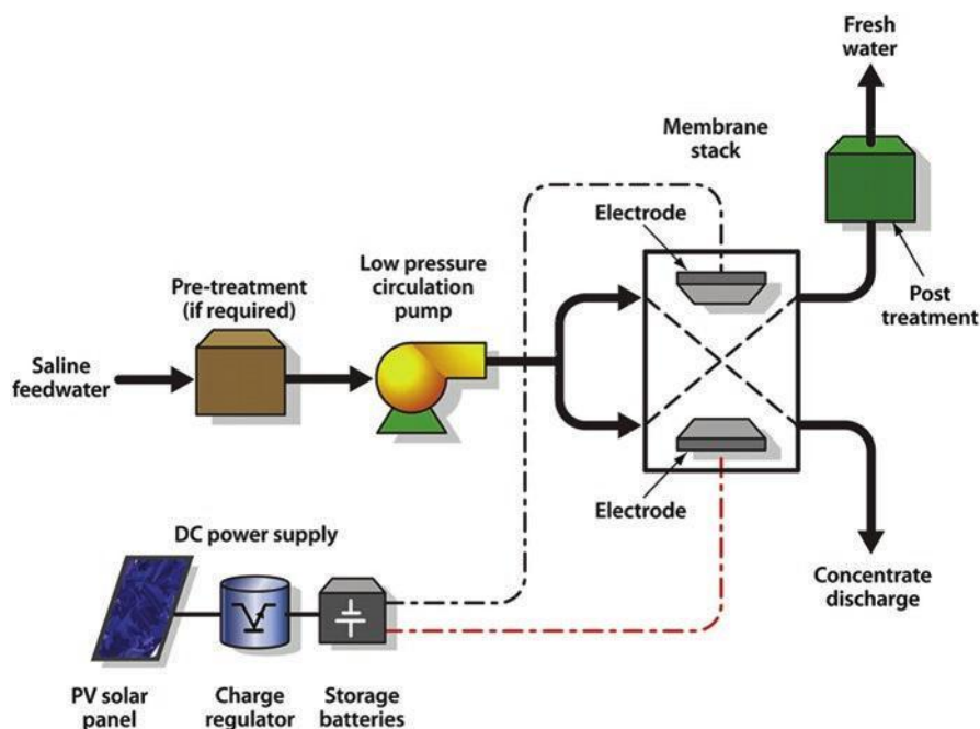
Fig. 7.8 A schematic diagram of a PV-ED system (Al-Karaghoul et al. 2010)
