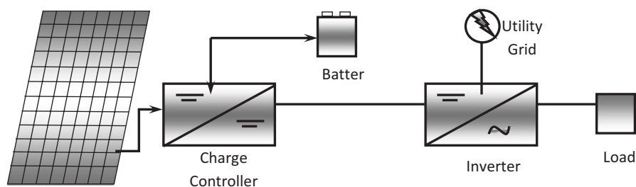
Fig. 7.1 Layout of a solar PV system
